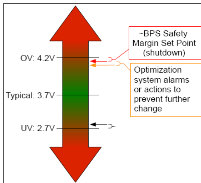
Figure 1 – Example Cell Voltage Operational Range
