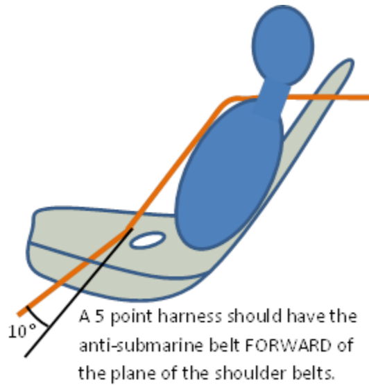
Figure 10.5a Configuration of anti-submarine belt attachment (5-point harness)
