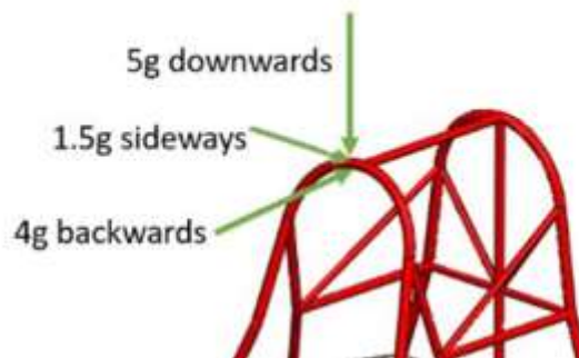
Figure 5 Combined Roll Cage Load Case (Front Hoop)
