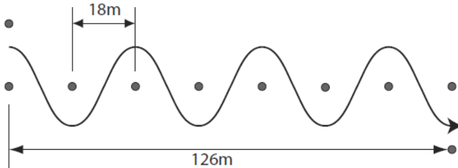
Figure 3 Slalom Course Layout
