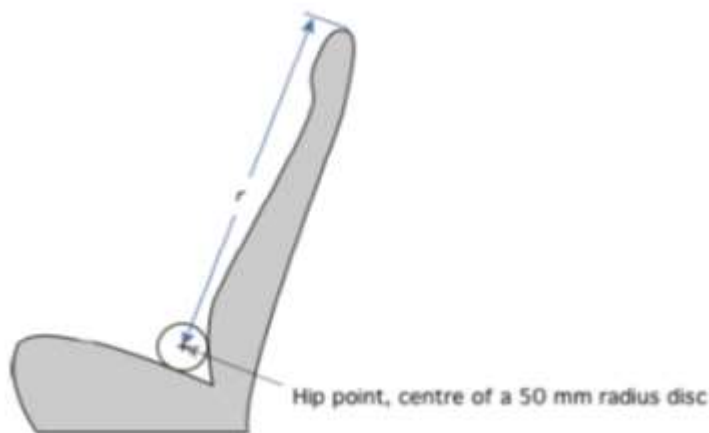
Figure 1 Hip Point Definition
